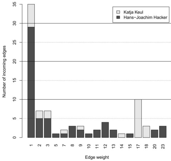
Figure 10: Homophily in the Linke network
