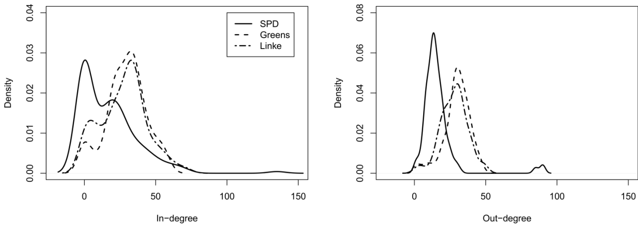
Figure 4: Degree distribution (Kernel Density Estimates)
